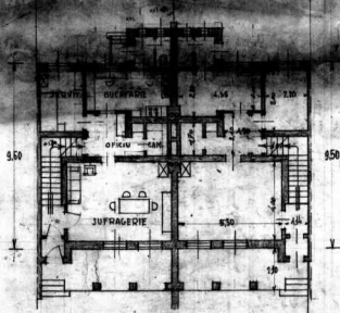
PLAN PARTER
